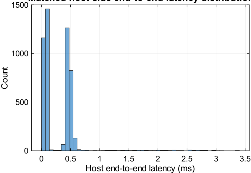
Matched host-side end-to-end latency distribution
